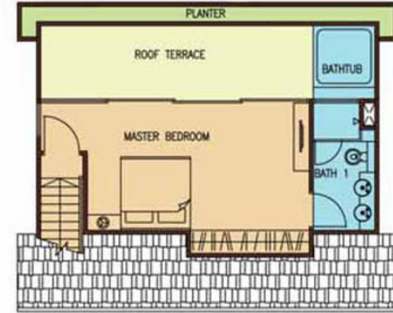
ATTIC PLAN
